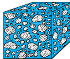
Poorly sorted sand
