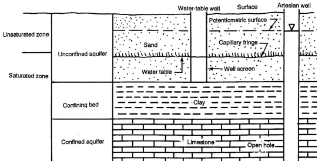
Figure 2-12. Unconfined aquifer
