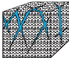
Fractures in granite
