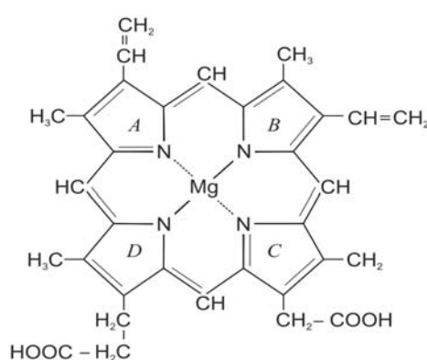
Clorofila
