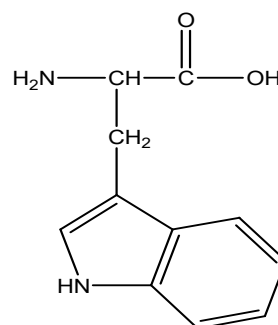
triptofan
