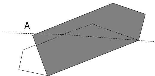
Fig. 7: Sfenoid
